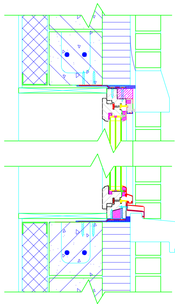
MASONRY CAVITY WALL
