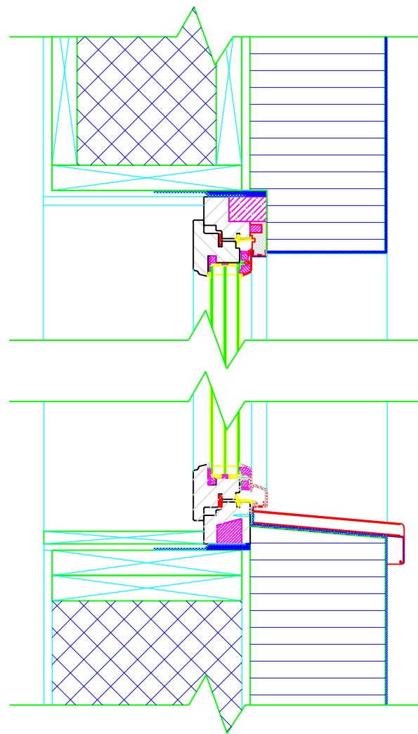
WOOD FRAME W/EFIS
