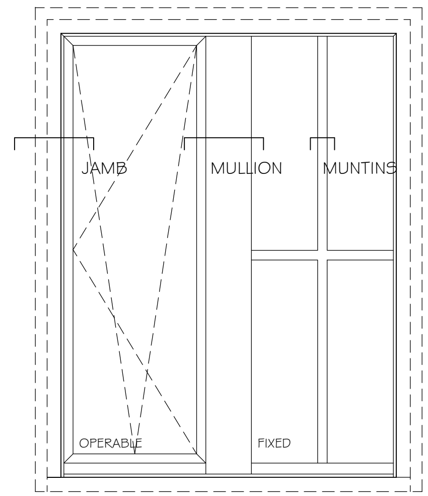
ELEVATION (FROM OUTSIDE) 1" = 1'-0"
